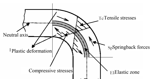
Fig. 1. Bending of sheet metal
