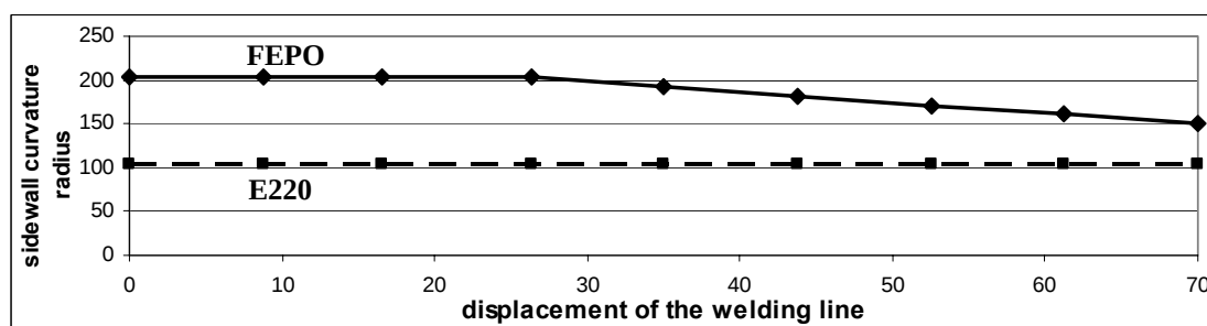
Fig. 11. Variation of sidewall curvature radius \rho
