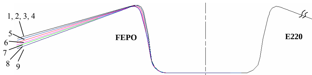
Fig. 8. Influence of the welding line position on springback of tailor welded strips
