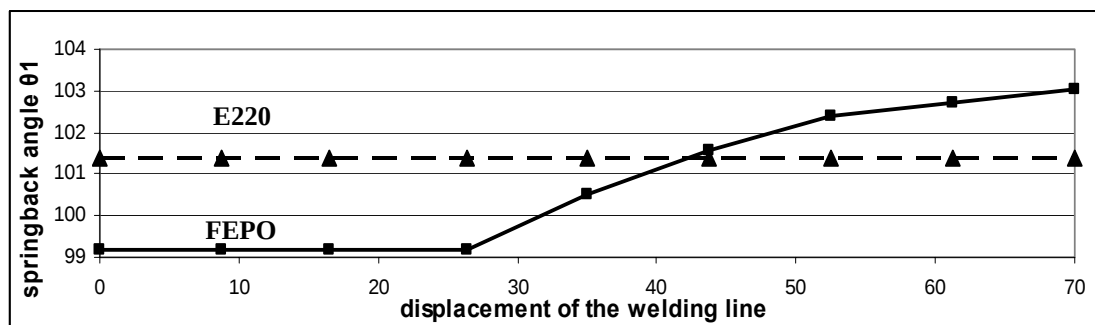
Fig. 9. Variation of angle \theta_1
