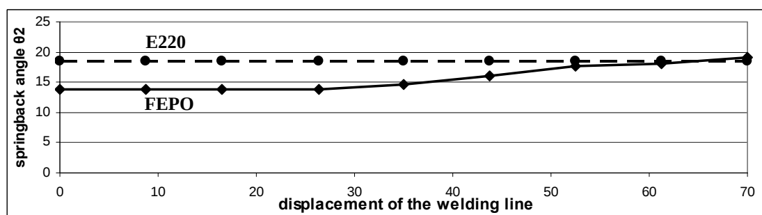
Fig. 10. Variation of angle \theta_2
