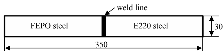
Fig. 2. Tailor welded strips for U-shape forming (unit: mm)
