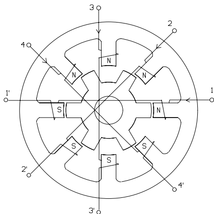
Fig.1. Structure of the SRM
