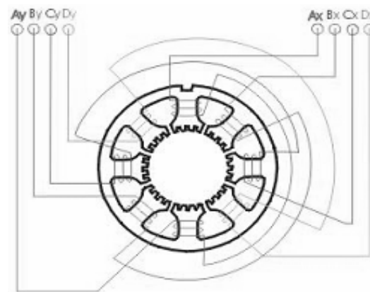
Fig. 2 Structure of the VRSM stator.
