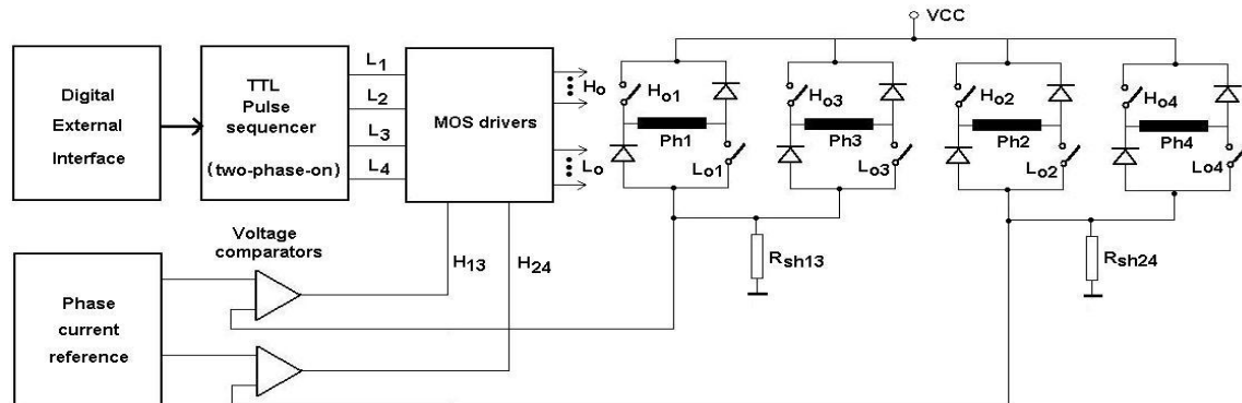
Fig. 5. Block diagram of the inverter
