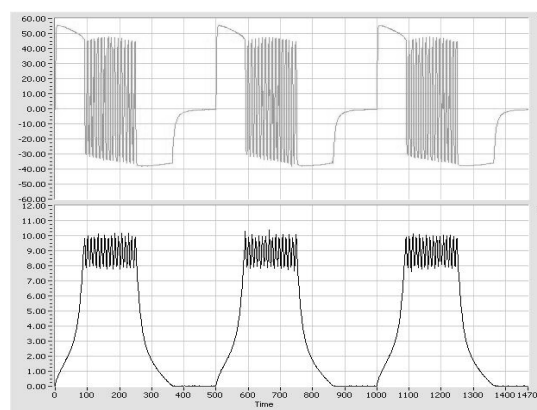
Fig. 9. Acquired voltage and current for SRM
