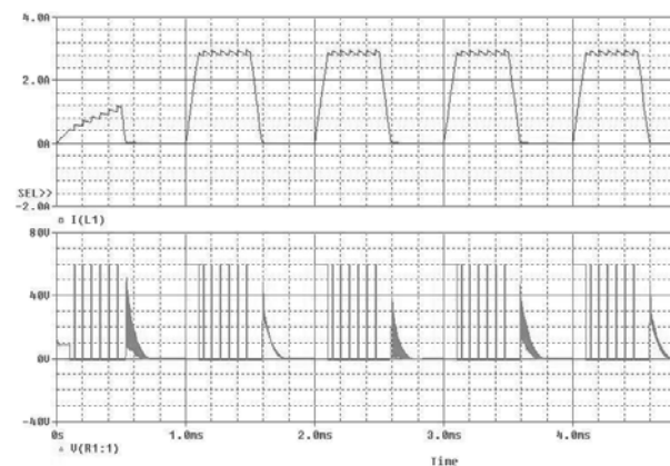
Fig. 7. Waveforms of PWM current and voltage. simulated in Pspice
