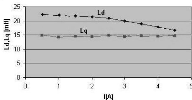
Fig. 4 Measured inductivities
