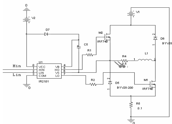
Fig. 6. OrCAD Capture model of the inverter
