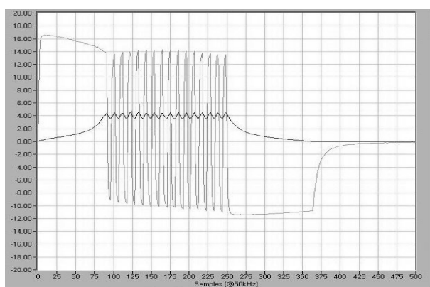
Fig. 8. Acquired waveforms of PWM current and voltage for VRSM
