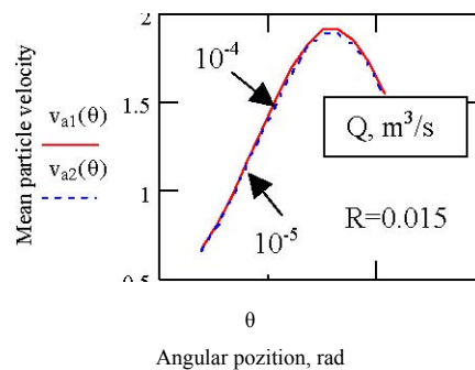
Fig.5. Mean velocity of the particle in gap.
