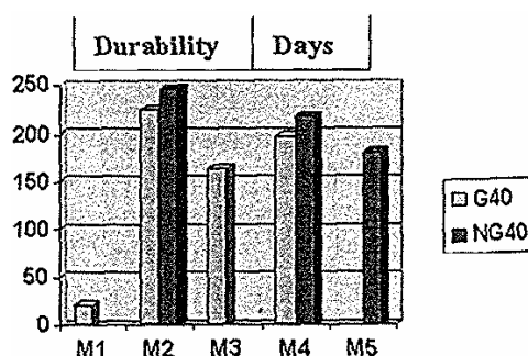
Fig.8 Durability of ball-valve pump
