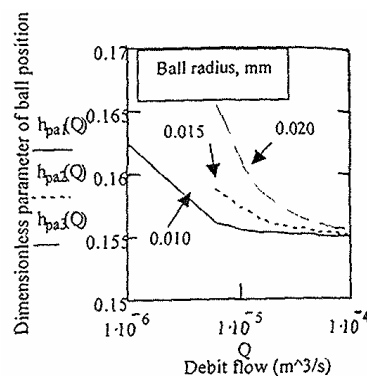
Fig. 2. Ball position in the conical gape.
