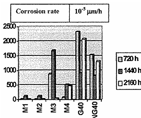
Fig.9 Corrosion rate of ball and seat materials
