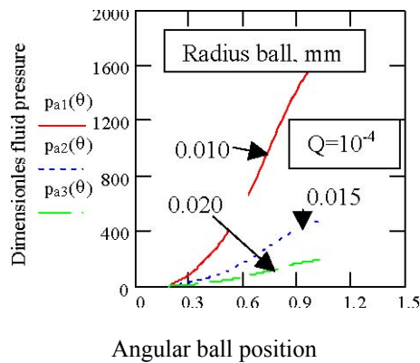
Fig.3 Fluid pressure in gap
