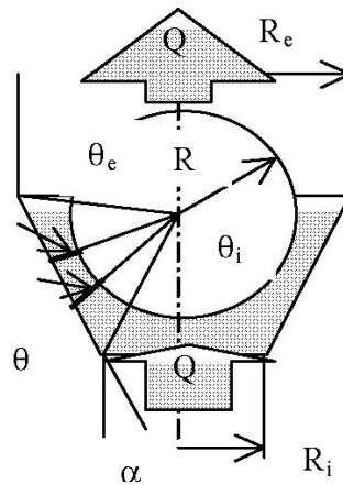
Fig.1. Geometry gapes for the flow model of crude petroleum liquid.
