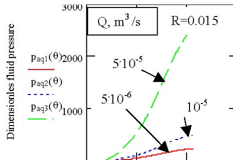
Fig.4 Fluid pressure in gap for diverse flow rates
