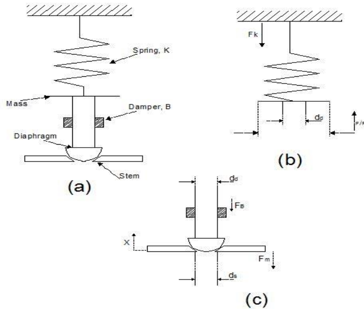
Fig. 1. Forces acting on globe valve system.
