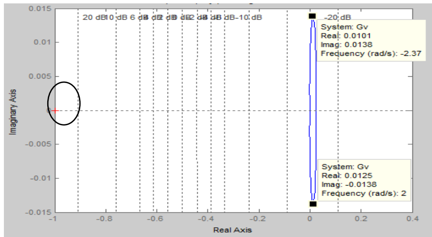
Fig. 4. Nyquist diagram of globe valve.
