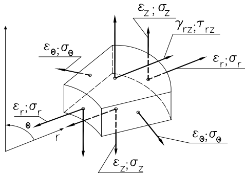
Fig. 3. Strains and curvatures in plane coordinate
